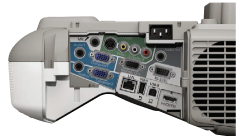
EB-475W interface
